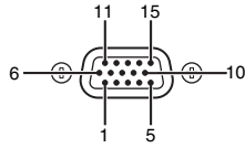
COMPUTER IN/OUT (Mini D-SUB 15-pin)
