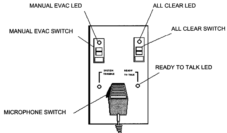
Figure 10. 4003 Audio Control Switches
