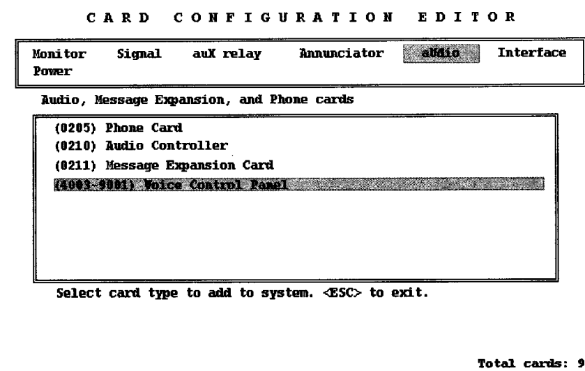
Figure 7. Adding the Voice Control Panel with the 4100 Programming Unit
