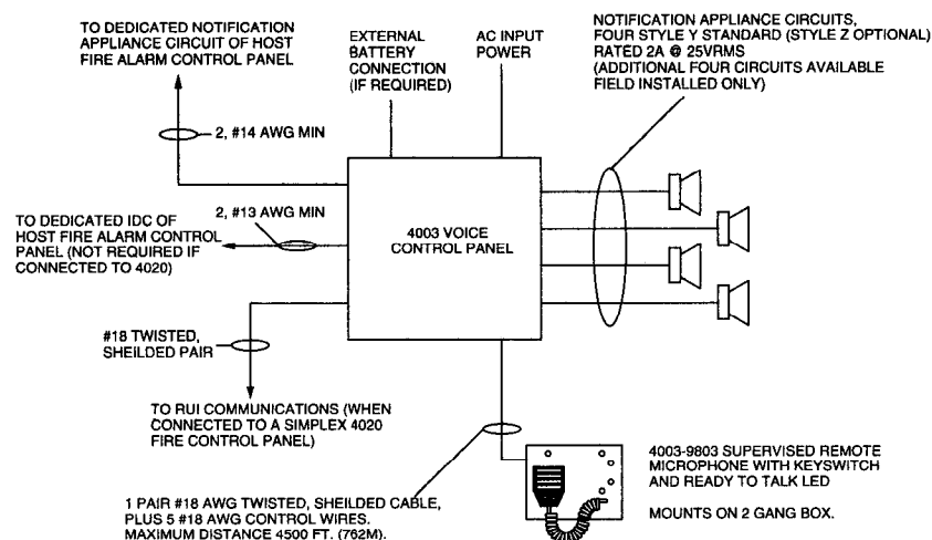
Figure 13. 4003 VCP Connection Diagram
