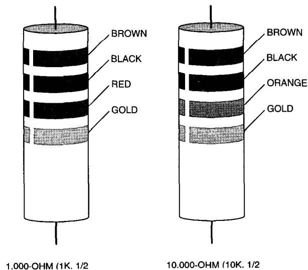
Figure 14. End-Of-Line Resistor Color Code
