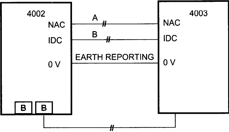
Figure 16. Interconnection to the 4002
