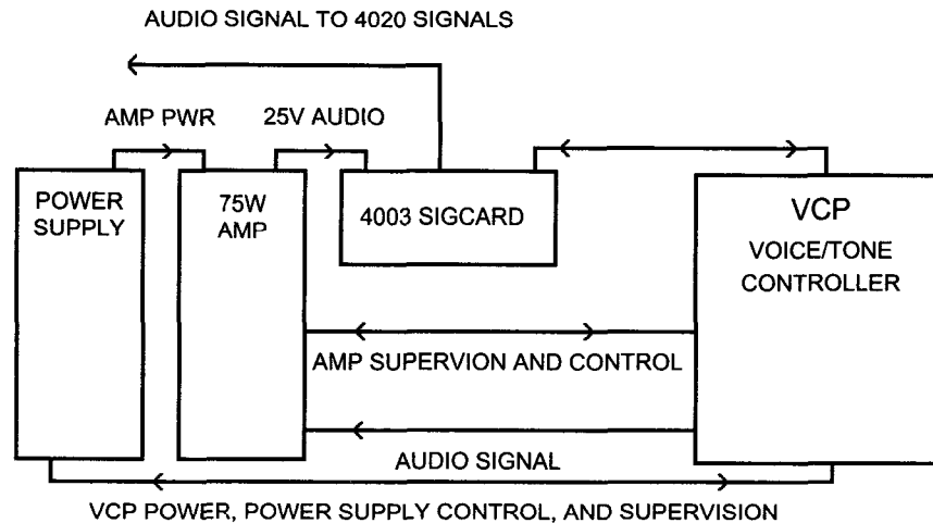
Figure 5. Voice Control Panel Functional Block Diagram
