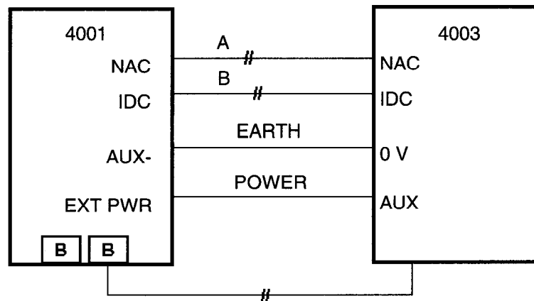
Figure 15. Interconnection to the 4001
