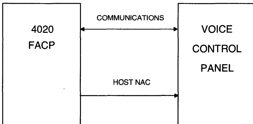
Figure 2. 4003 Voice Control Panel in the Slave Configuration
