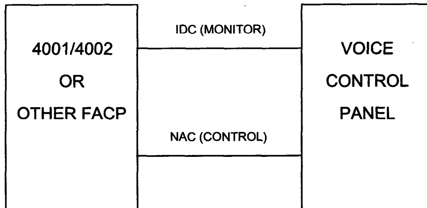
Figure 3. 4003 Voice Control Panel in the Adjunct Configuration
