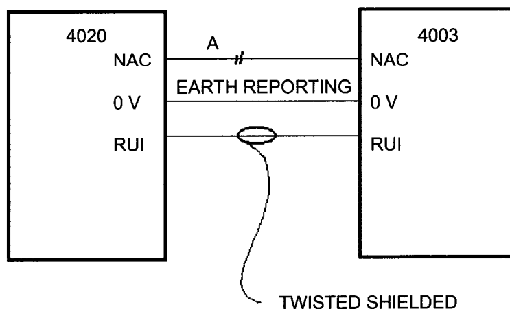
Figure 17. Interconnection to the 4020
