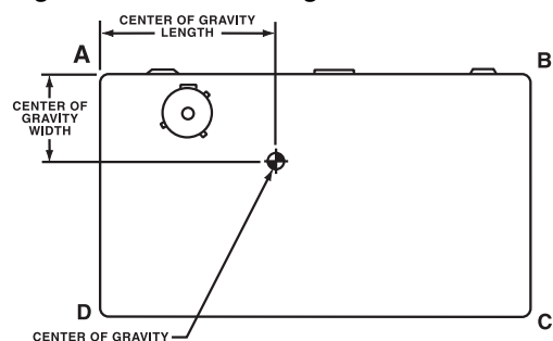
Figure 6. Corner weights
