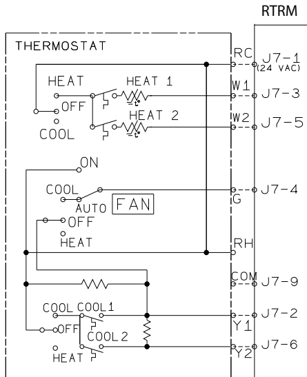
Figure 28. Typical field wiring diagrams for Electro Mechanical
