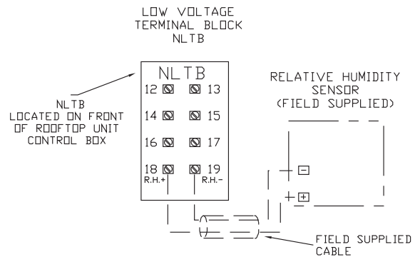
Figure 30. ReliaTel relative humidity sensor (dehumidification option)
