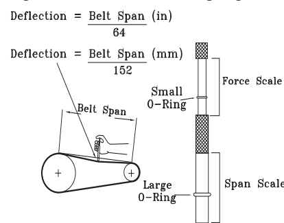
Figure 40. Belt tension gauge
