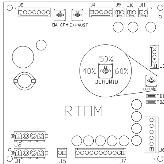
Figure 29. ReliaTel options module
