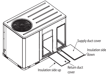
Figure 19. Duct cover
