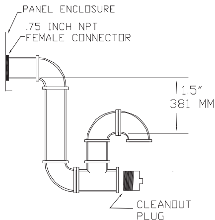
Figure 25. Condensate trap installation
