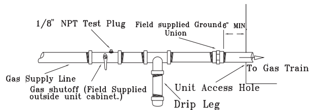
Figure 38. Schematic diagram for filed gas piping to unit
