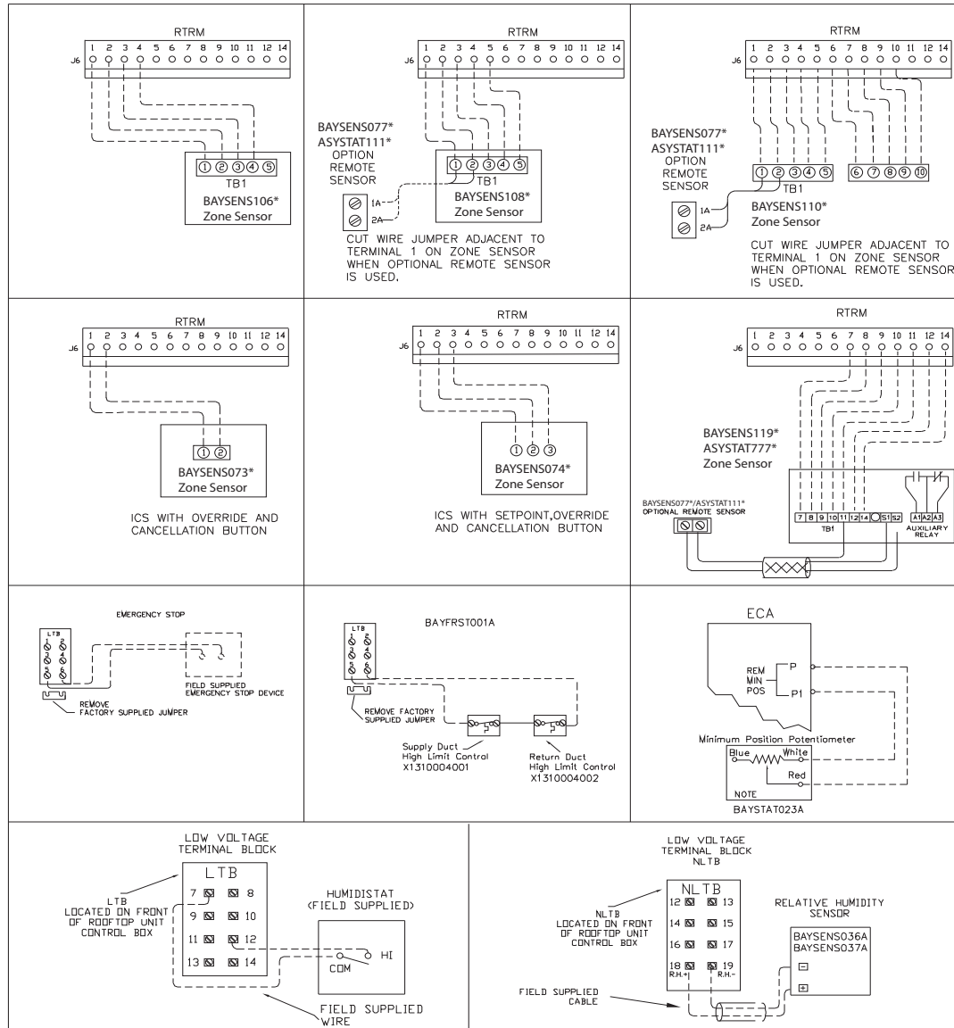
Figure 37. Typical field wiring diagrams for optional controls (ReliaTel only)
