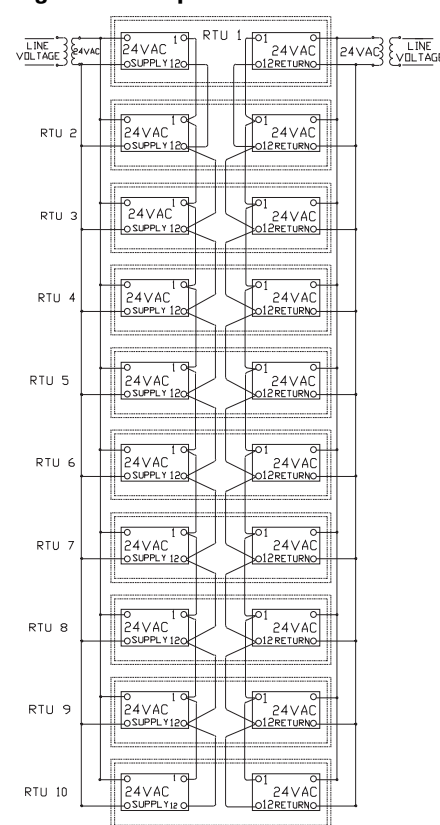
Figure 35. Up to 10 HVAC units
