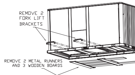
Figure 12. Fork pocket
