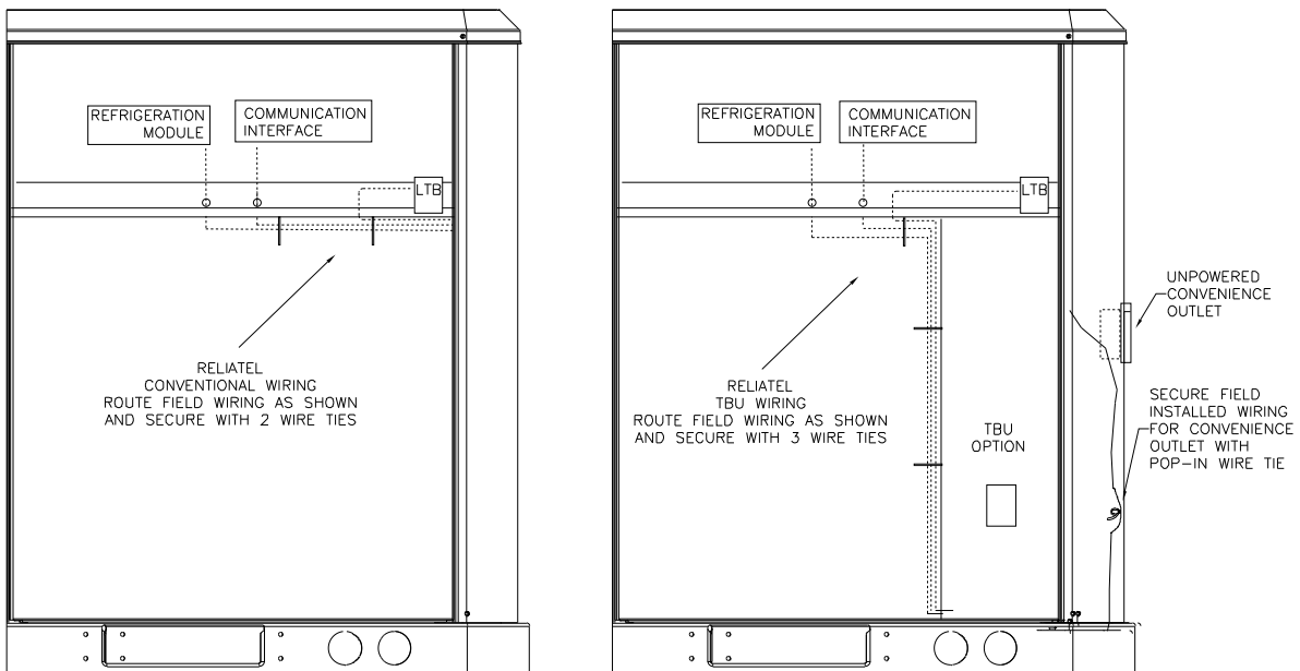
Figure 33. ReliaTel control customer low voltage routing
