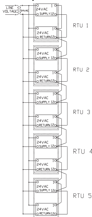
Figure 34. Up to 5 HVAC units
