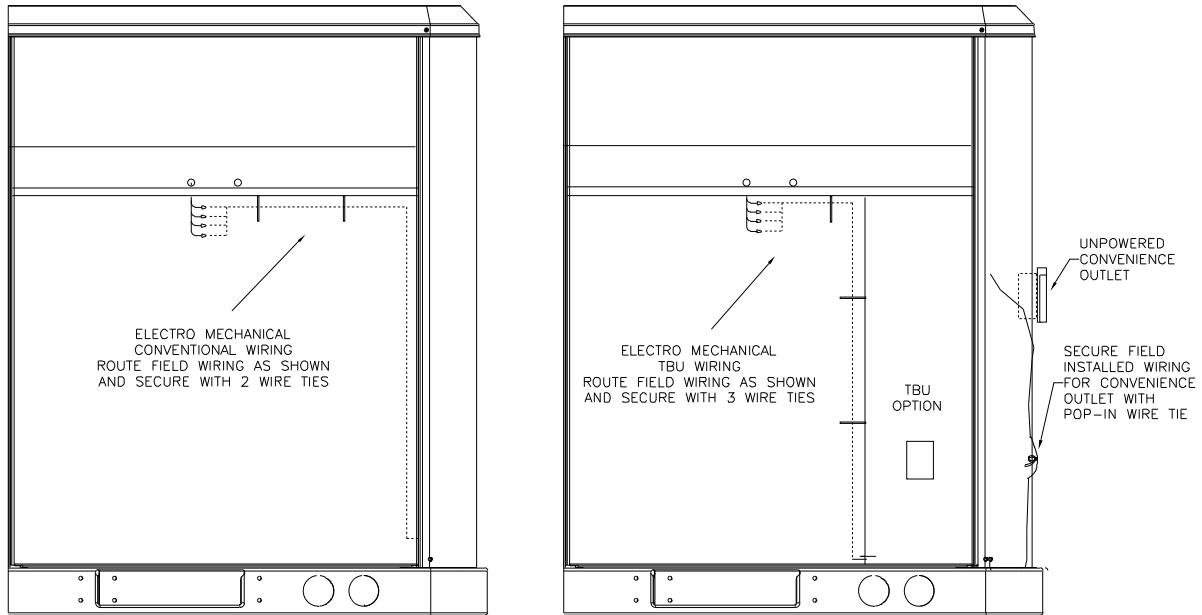
Figure 32. Electro mechanical control customer low voltage routing
